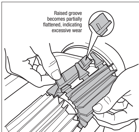
Figure 18. Worn Brush Indicator
