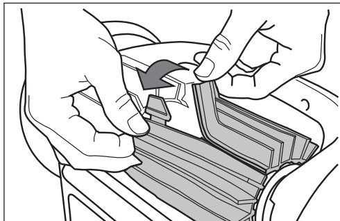
Figure 20. Undo the Tabs of the Brush
