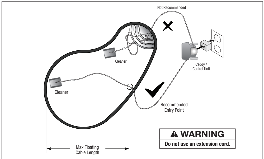
Figure 6. Pool Entry Point for Optimal Patterning
