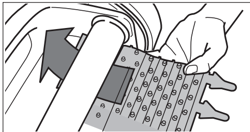
Figure 21. Position the New Brush on Roller
